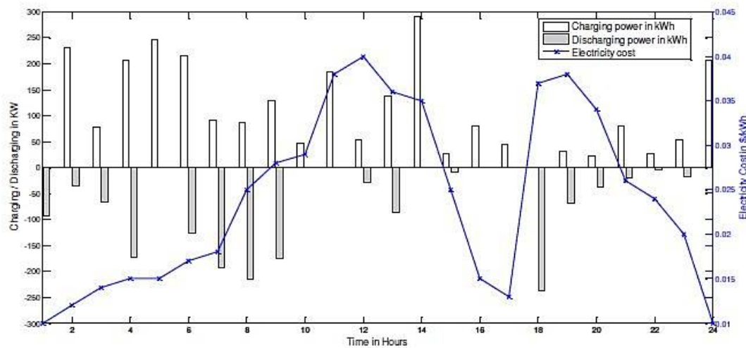
Figure 9 Charging and discharging power in case2
