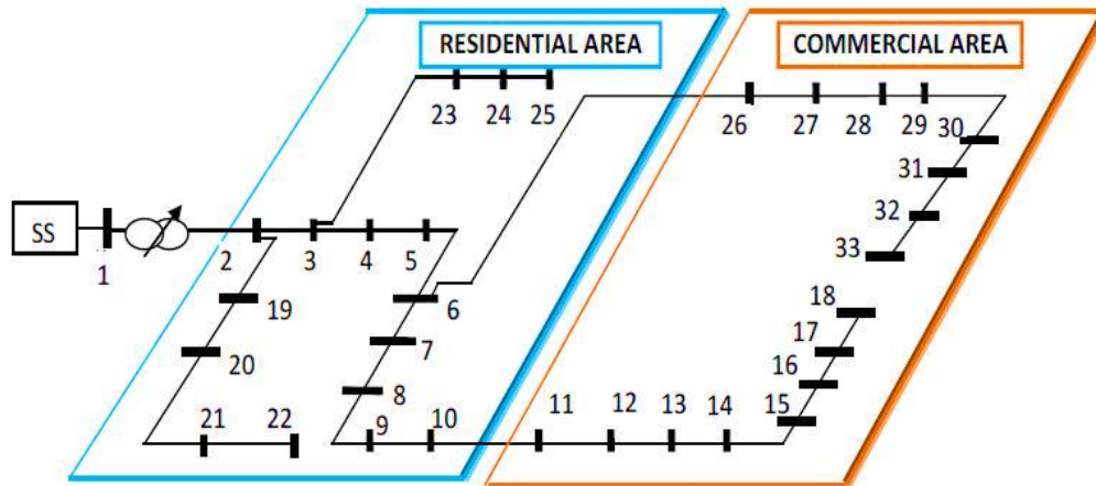
Figure 6. IEEE 33-bus distribution model with two zones
